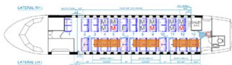
ATR 42 typical 3 stretchers version
